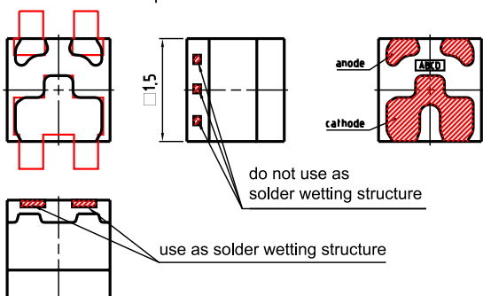
Component Location on Pad
